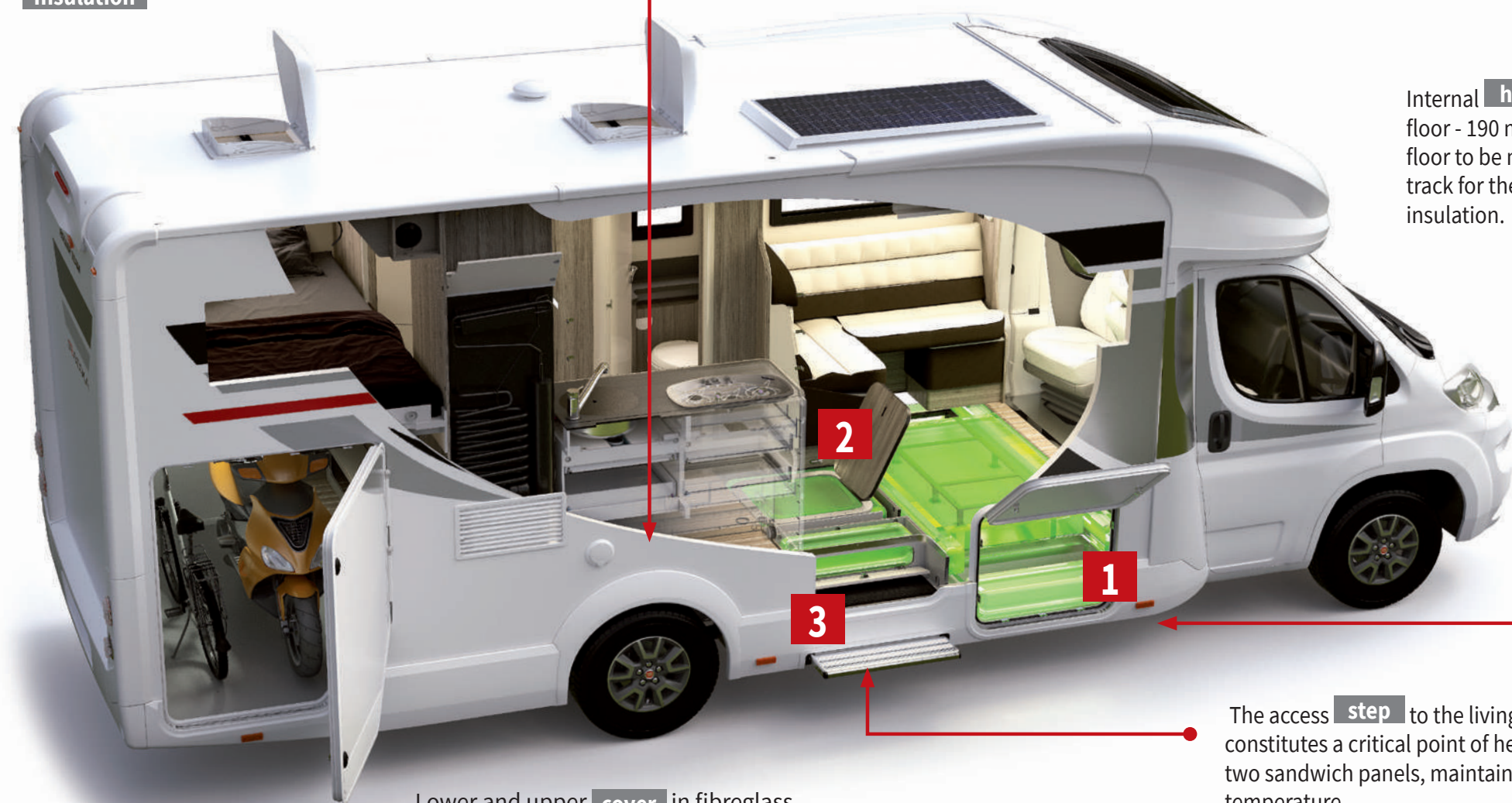
1 Through-floor maxi-garage 550 l
